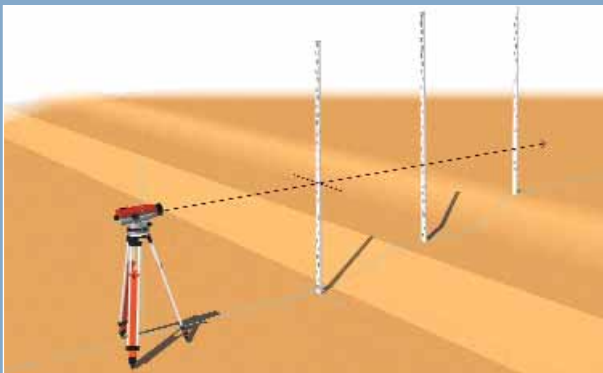
Elevations
